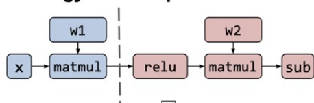
Strategy 1: Inter-operator Parallelism
