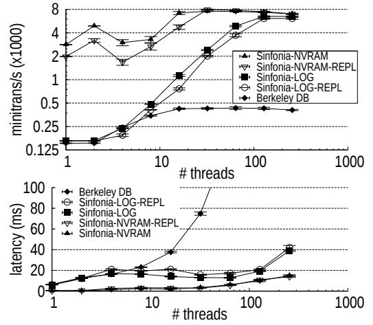
Figure 12: Performance of Sinfonia with 1 memory node.
