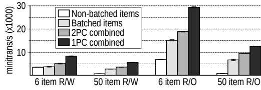
Figure 13: Performance with various combinations of techniques.
